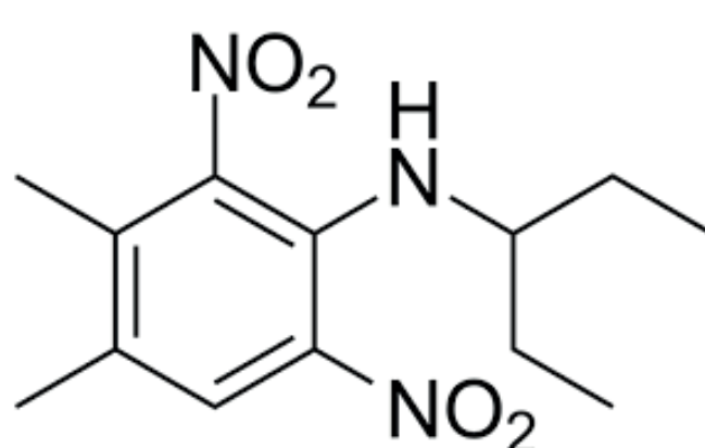
Pendimethalin
