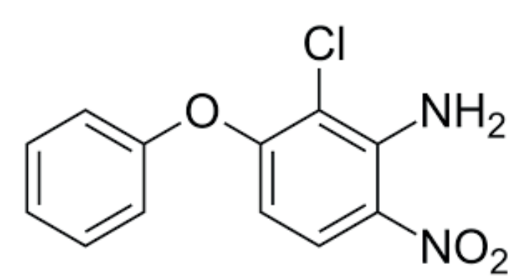
Aclonifen
