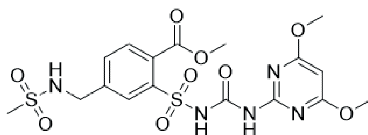
Mesosulfuron-methyl
