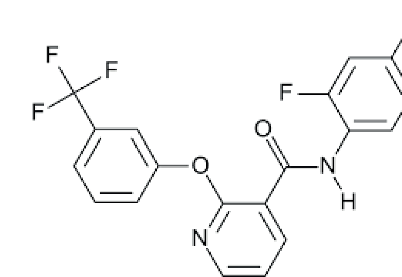
Diflufenican
