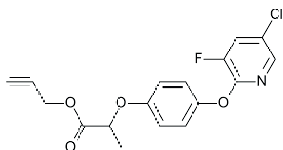
Clodinafop-propargyl
