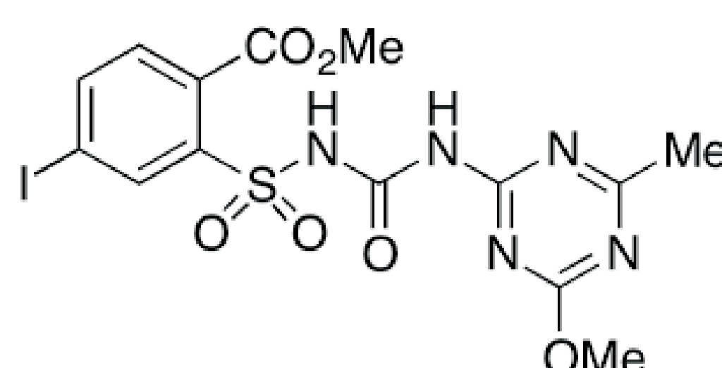
Iodosulfuron-methyl
