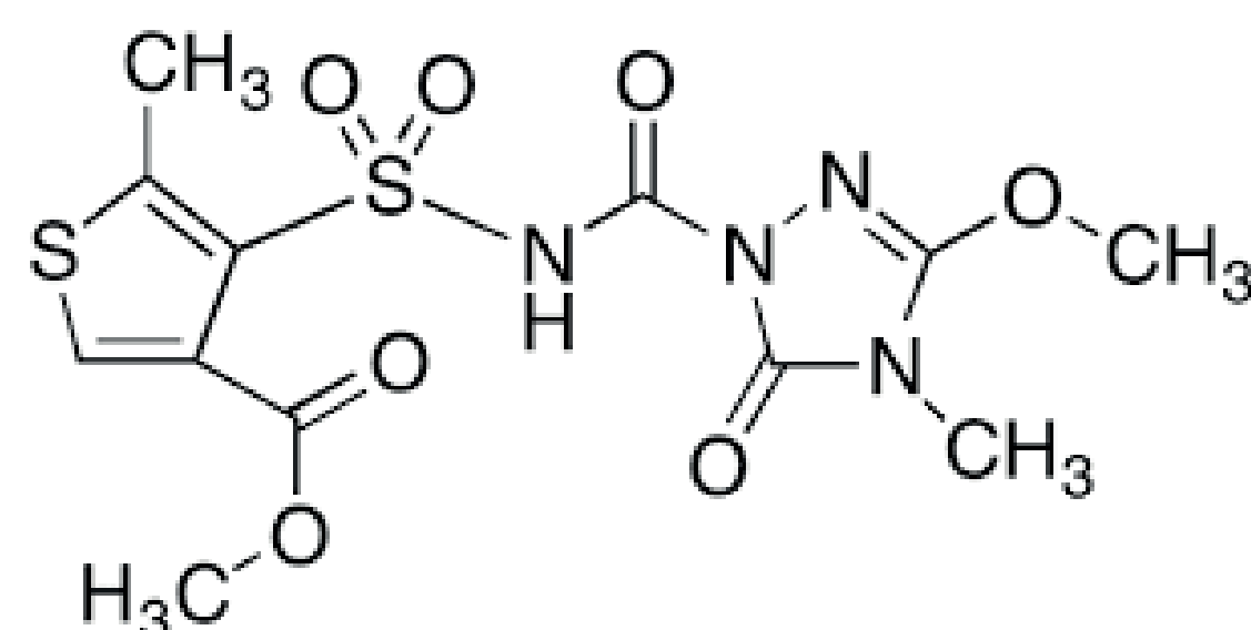
Pyroxsulam
